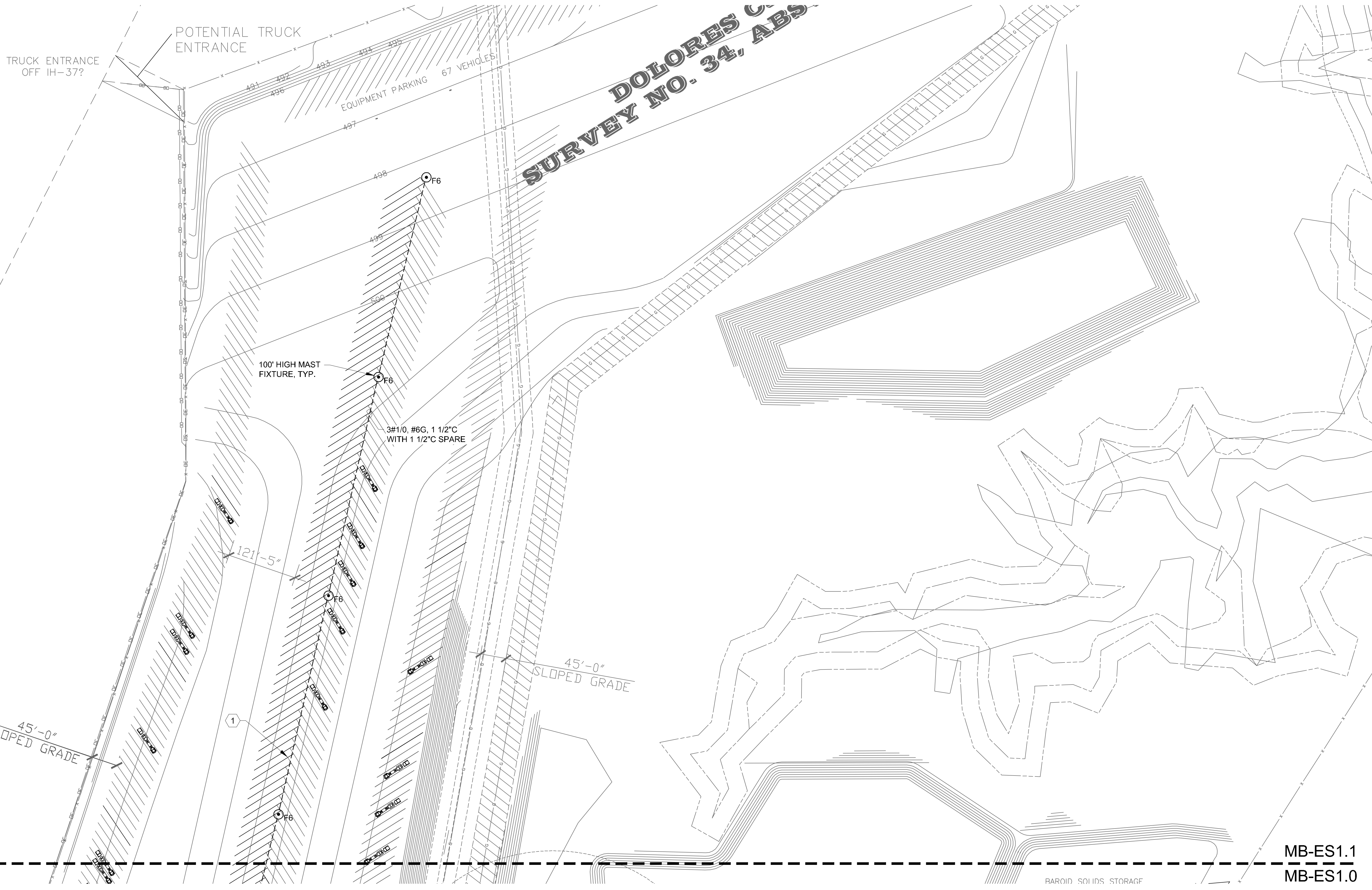
1 ELECTRICAL SITE PLAN MB-ES1.1 SCALE: 1" = 80'-0"
